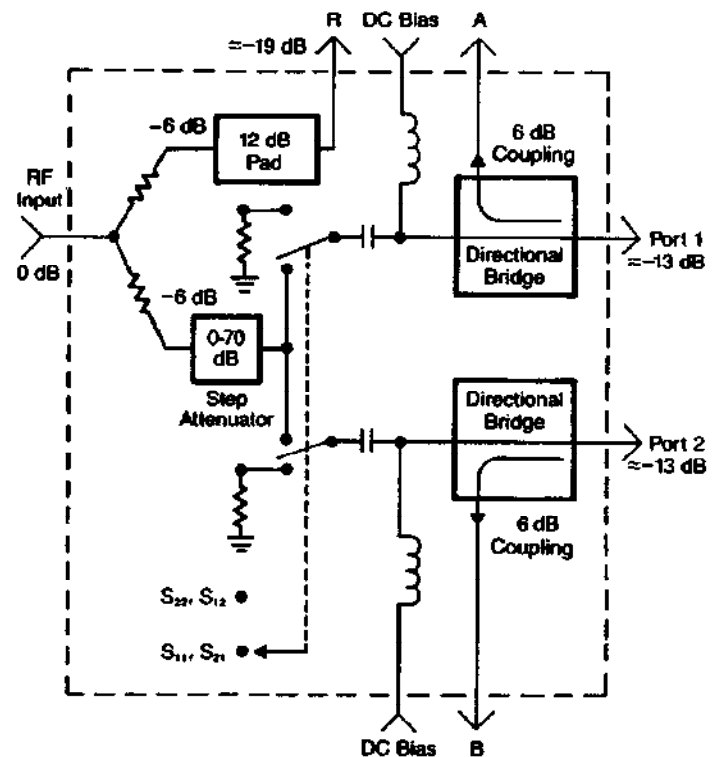
HP 85046A Schematic
