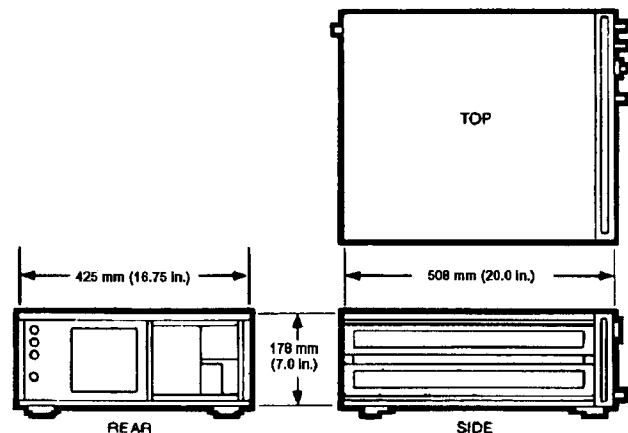
HP 8752C physical dimensions
