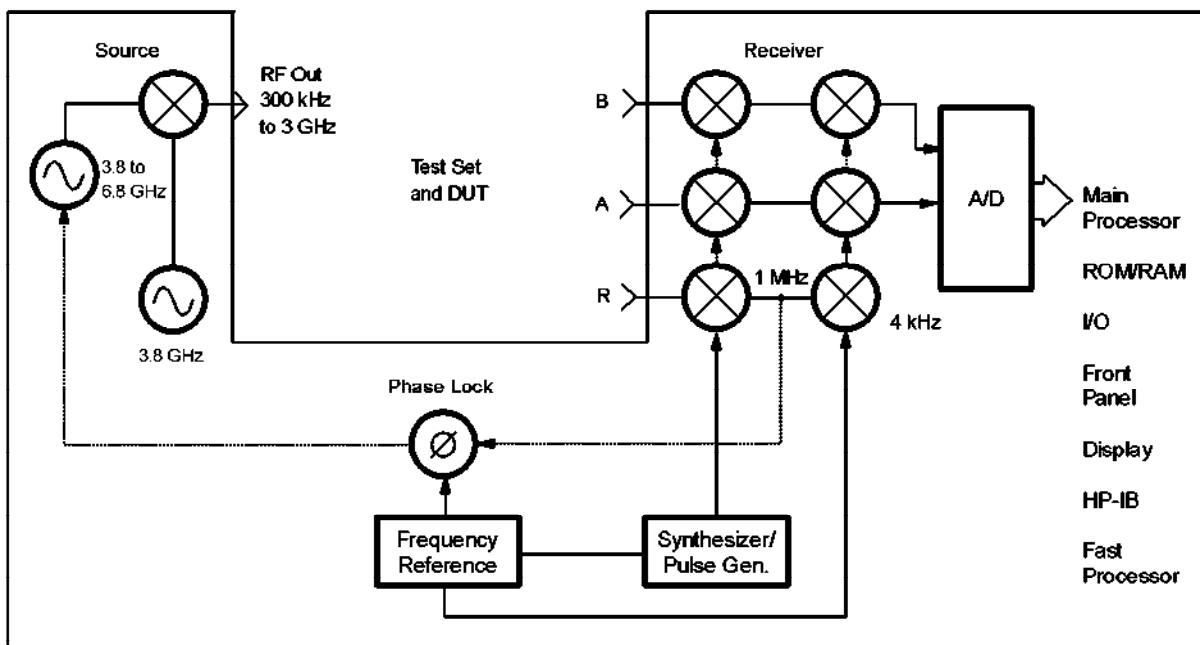
HP 8753D Option 011 Block Diagram
