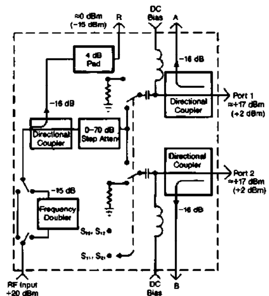
HP 85047A Schematic
